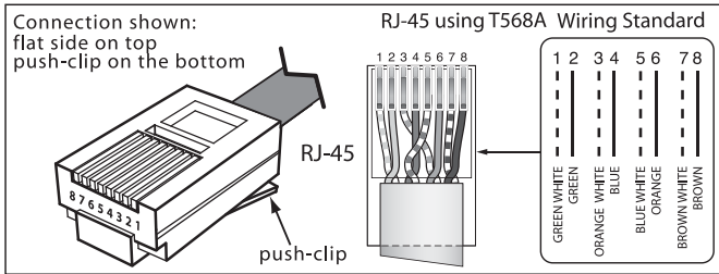
RJ-45 Connection Details
